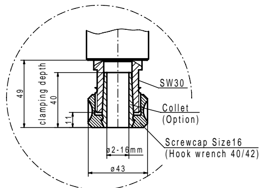
Collet receptacle Size 16
